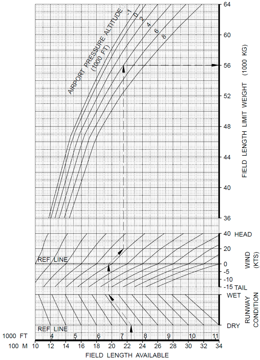
Figure 6: Example of interpolating between lines in a landing distance performance graph.
