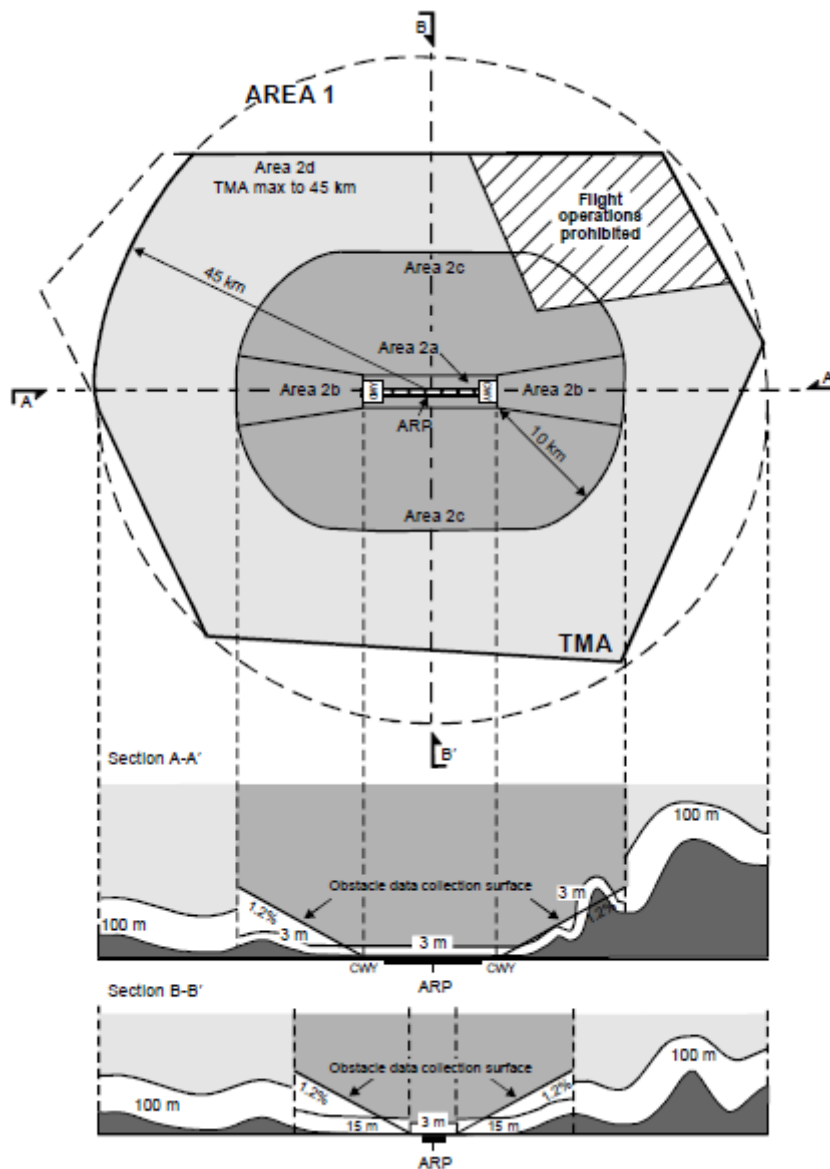
Figure 2 - Obstacle data collection surfaces — Area 1 and Area 2
