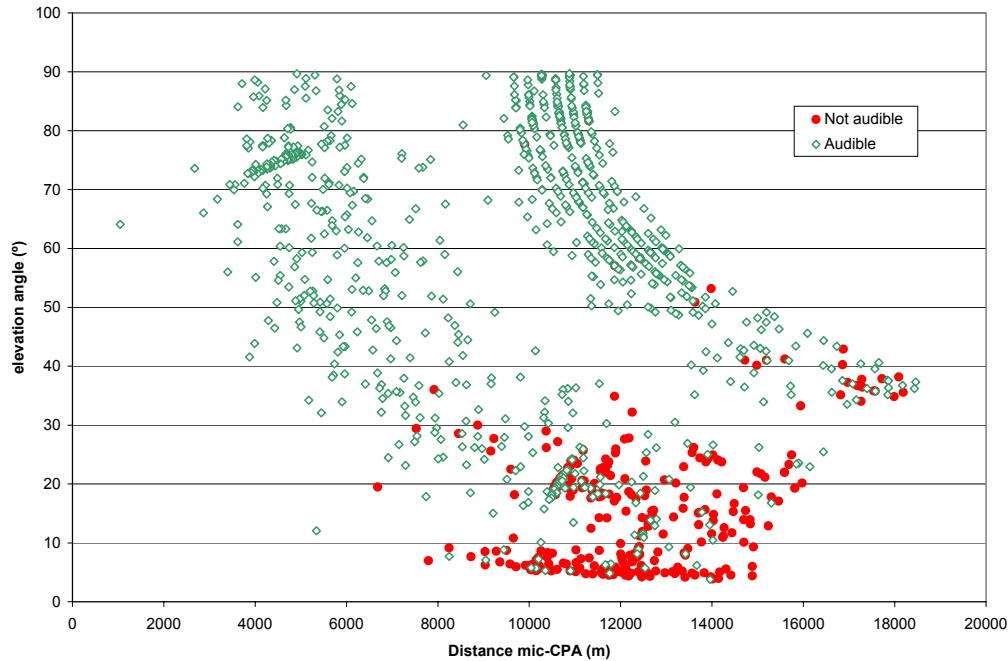
Figure 4- 11 Audibility related to distance and elevation angle
