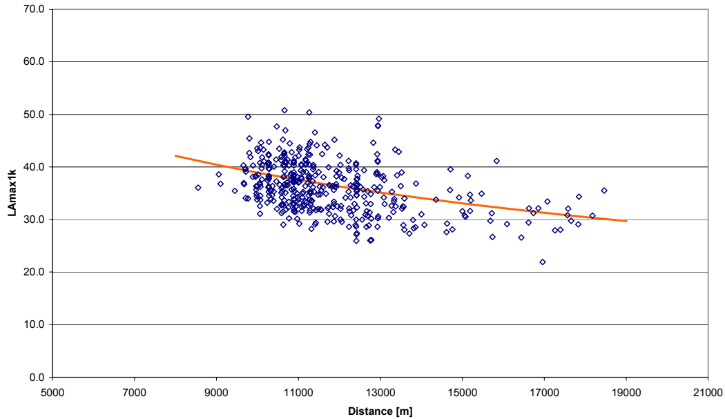
Figure 6- 8 Emperical model for MR2 – Cruise – LAmax1k inverted mic
