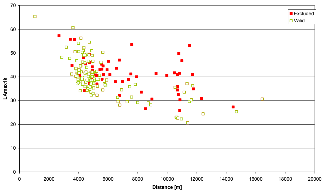
Figure 6- 26 L Amax1k for all valid aircraft events (DESCENT phase)
