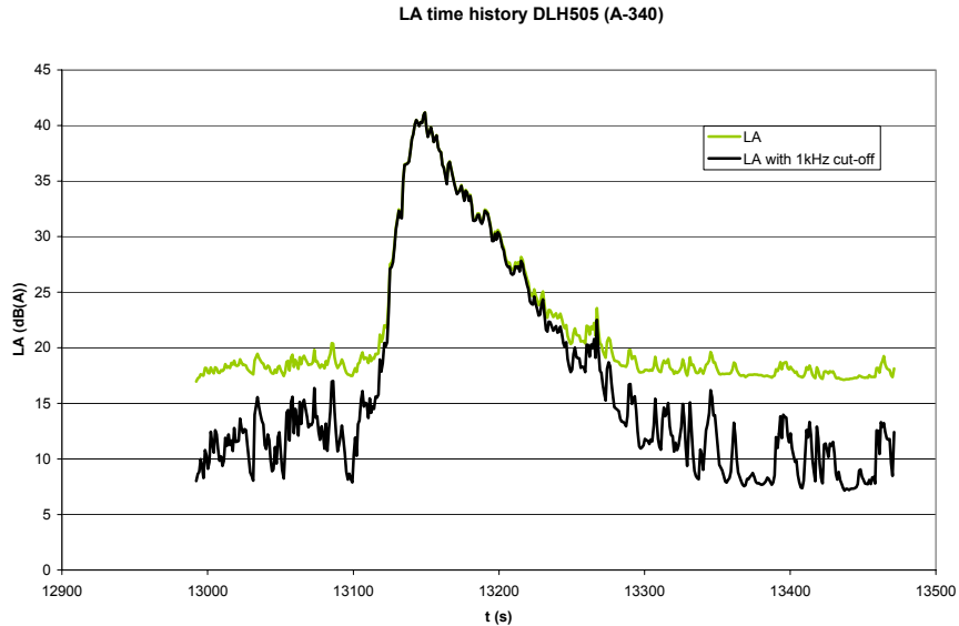
Figure 4- 6 Coincidence of LA and LA1k metrics during the event
