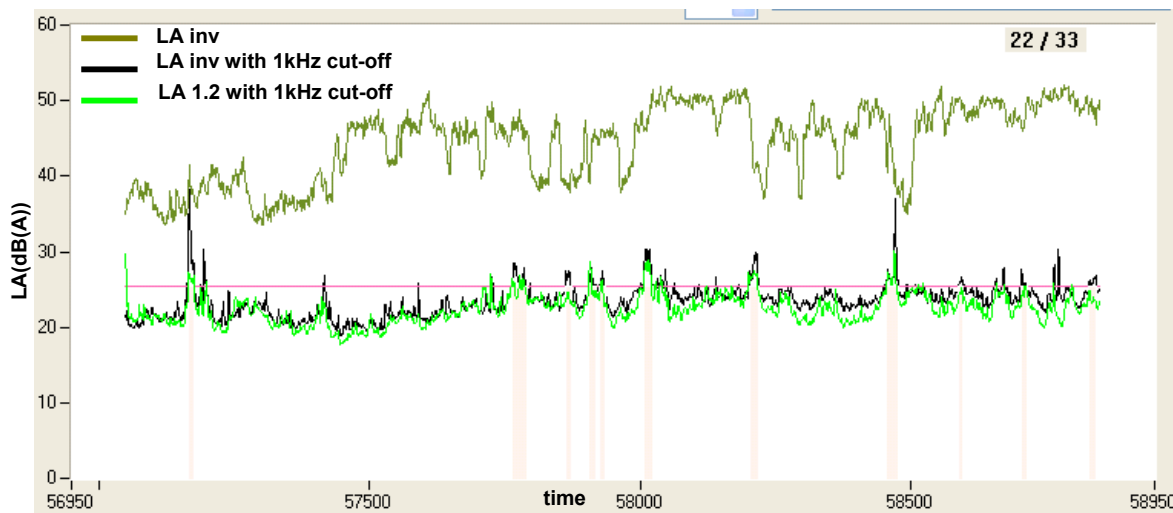
Figure 5- 12 Example of day-time measurement at Los Tablones with cicadas
