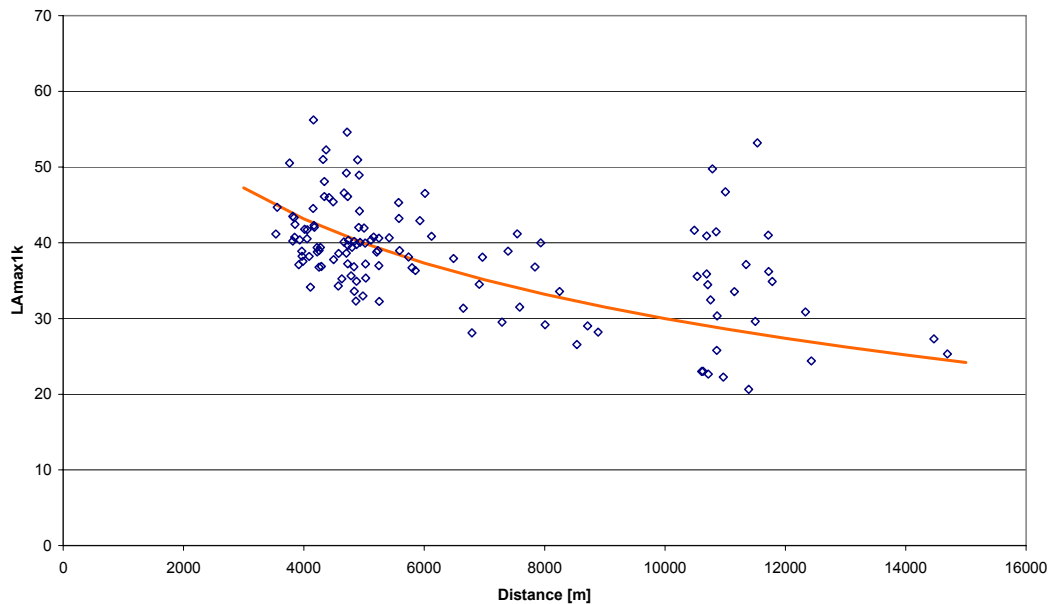
Figure 6- 9 Emperical model for MR2 – Descent – LAmax1k inverted mic
