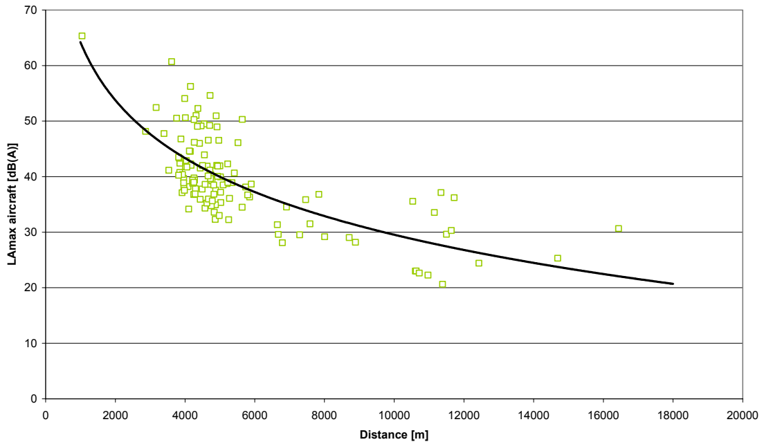
Figure 6 LAmax for all valid jet aircraft events (DESCENT phase)
