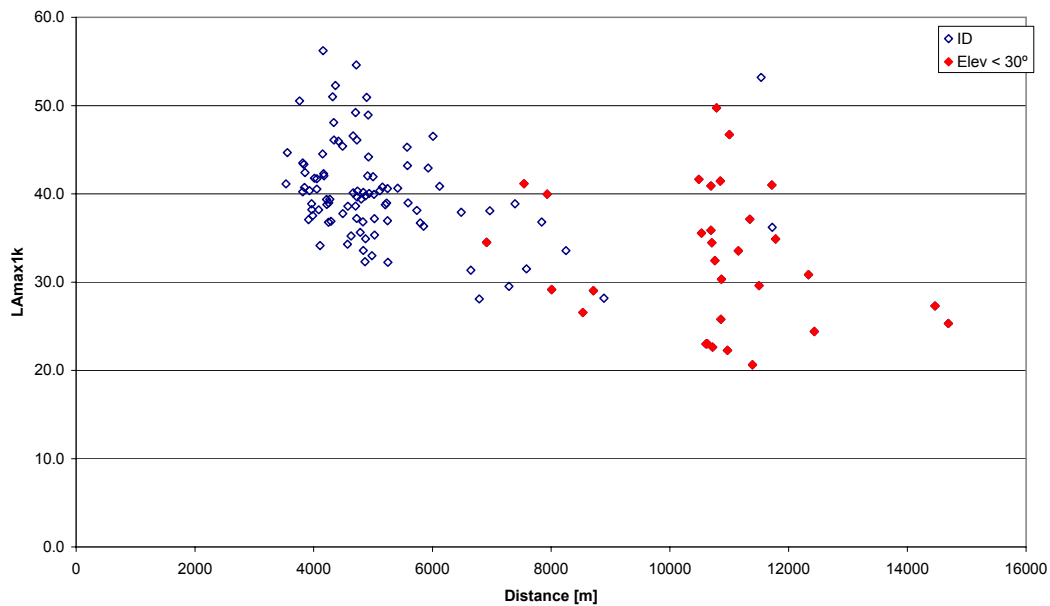
Figure 6- 19 Elevation angle: MR2-Descent-LAMAX1k inverted mic
