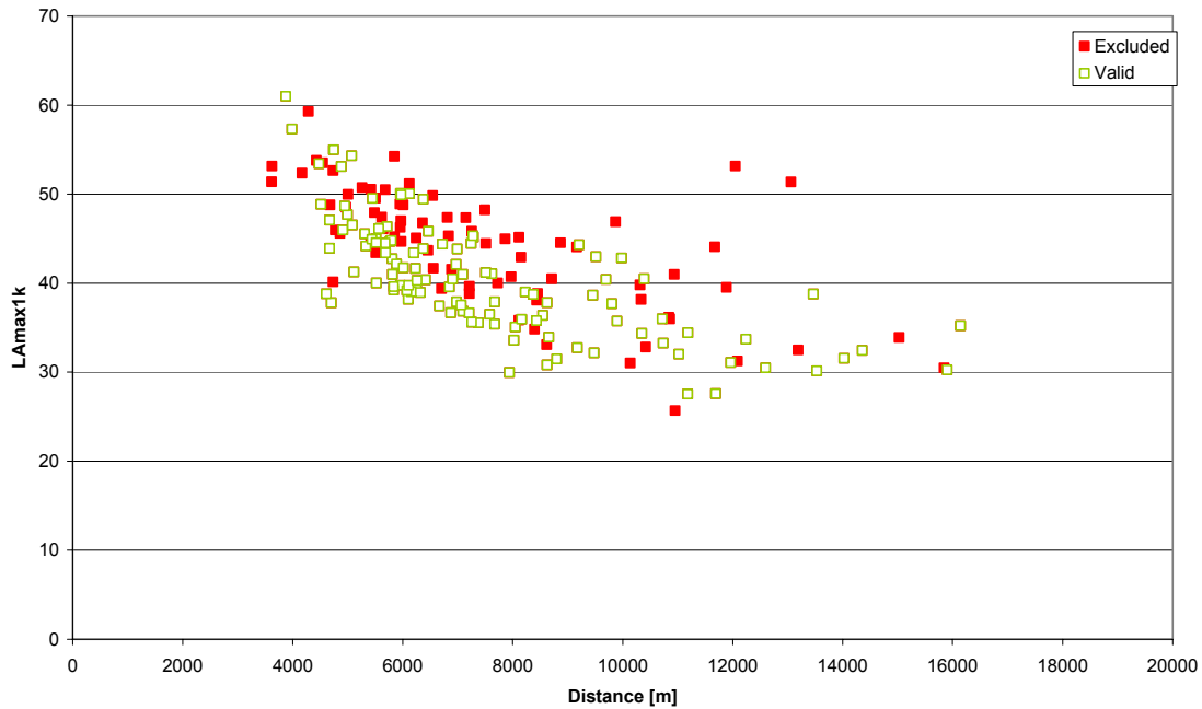
Figure 6- 24 L Amax1k for all valid aircraft events (CLIMB phase)
