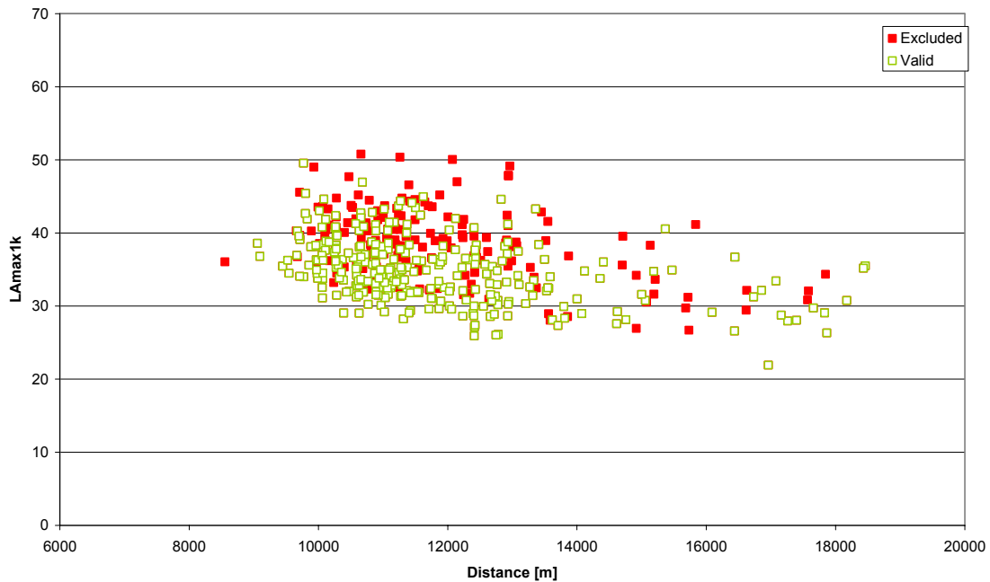
Figure 6- 25 L Amax1k for all valid aircraft events (CRUISE phase)
