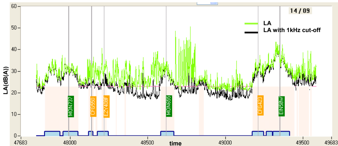
Figure 4- 3 Typical measurement
