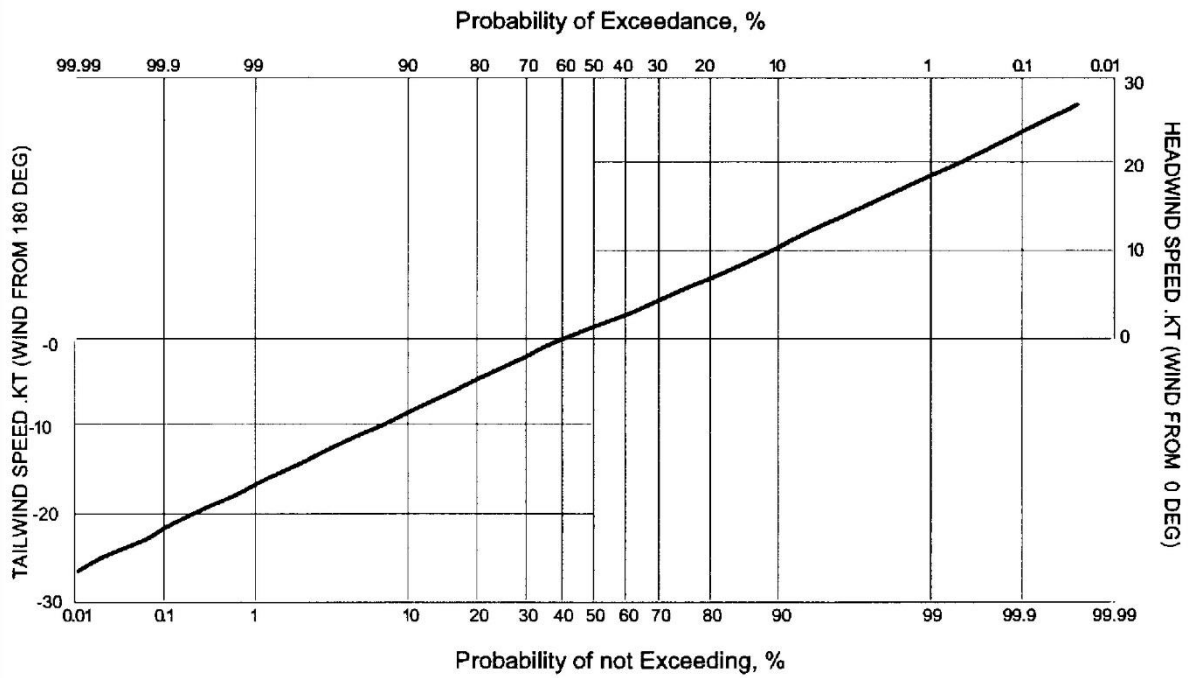
FIGURE 2 Headwind – Tailwind Description
