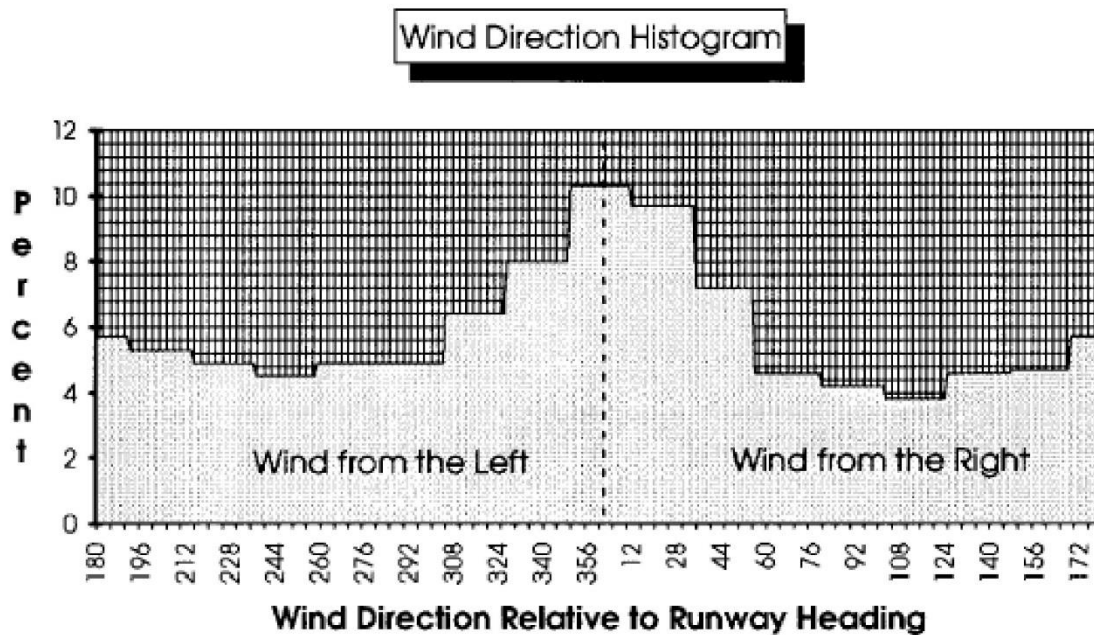
FIGURE 5 Wind direction relative to Runway Heading
