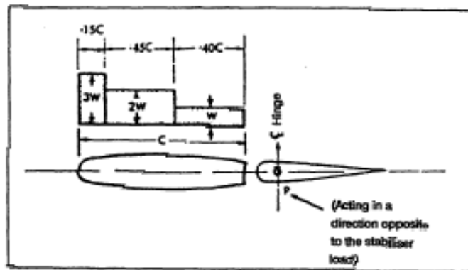
FIGURE B6 - TAIL SURFACE LOAD DISTRIBUTION.
