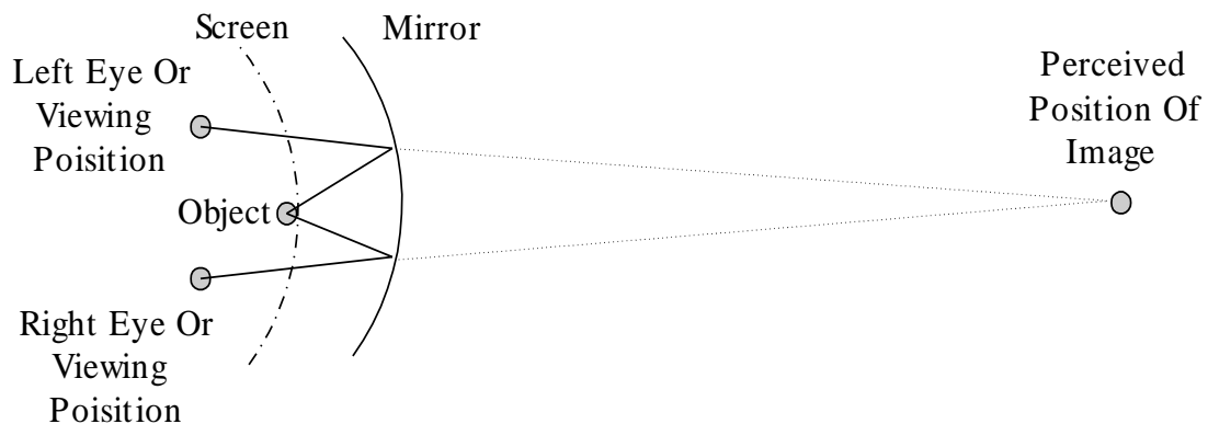
Figure 1: Collimated display
