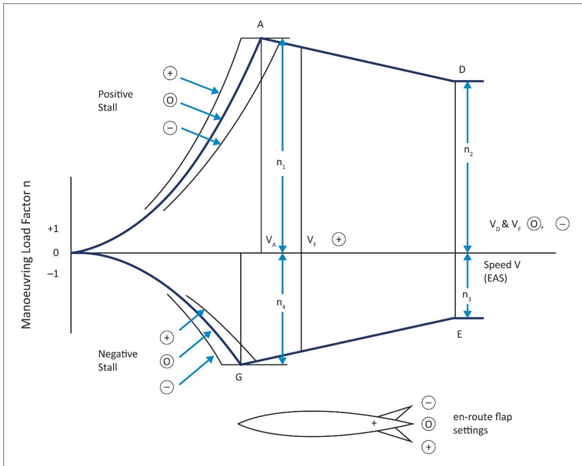
Figure 1 MANOEUVRING ENVELOPE
