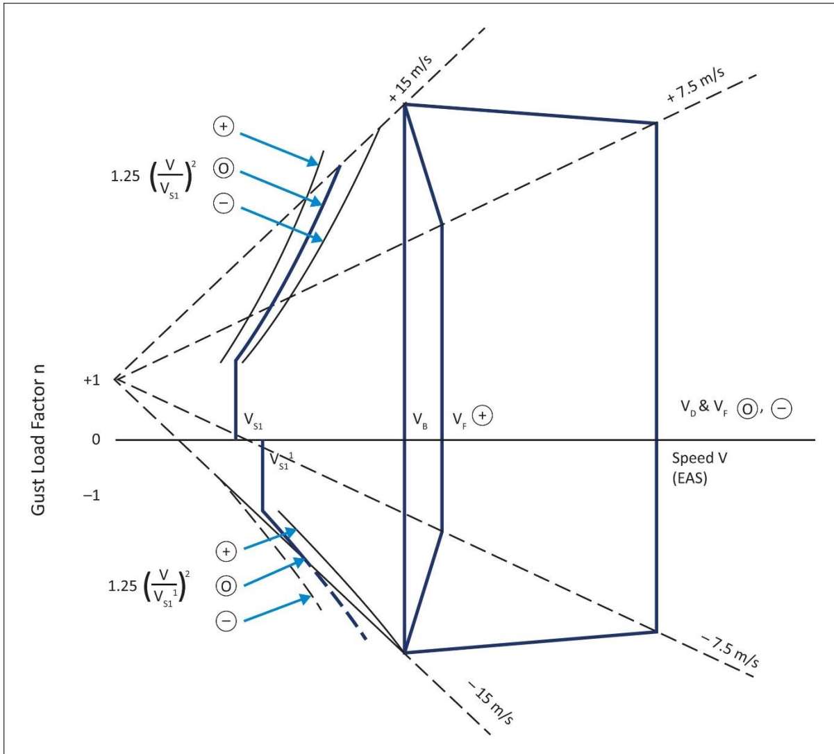
Figure 2 GUST ENVELOPE
