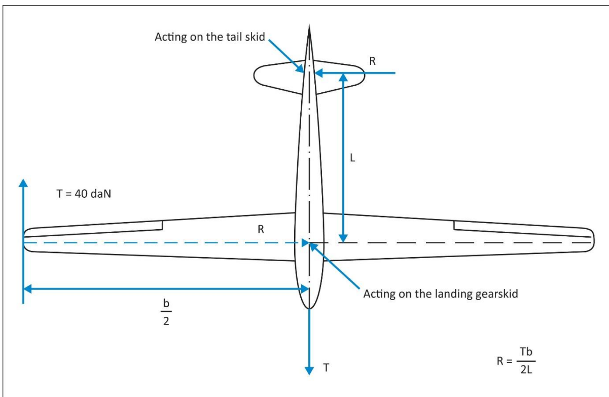
Figure 4 WING-TIP LANDING
