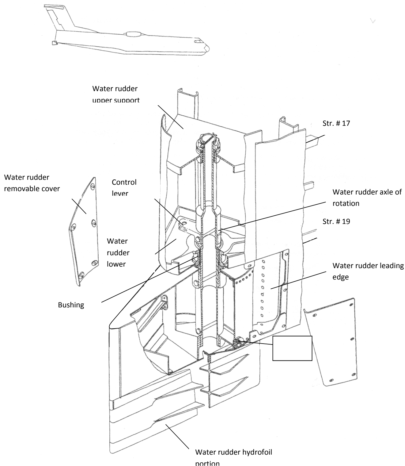
Fig. 1 Water rudder.
