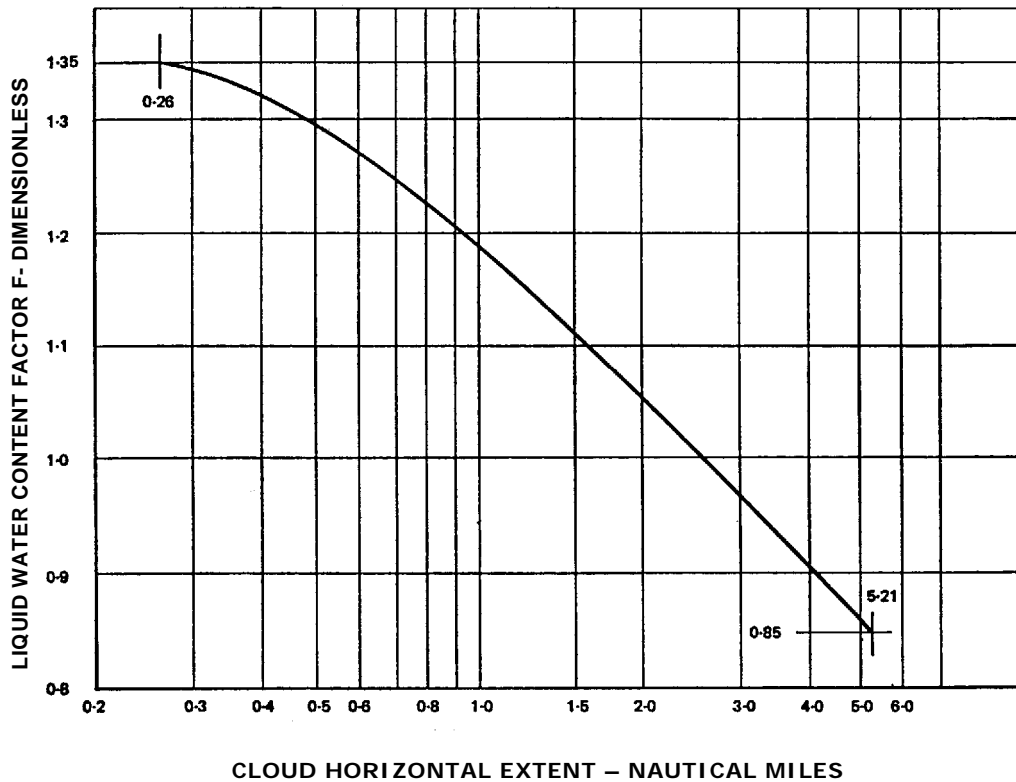
INTERMITTENT MAXIMUM (CUMULIFORM CLOUDS) ATMOSPHERIC ICING CONDITIONS VARIATION OF LIQUID WATER CONTENT FACTOR WITH CLOUD HORIZONTAL EXTENT
