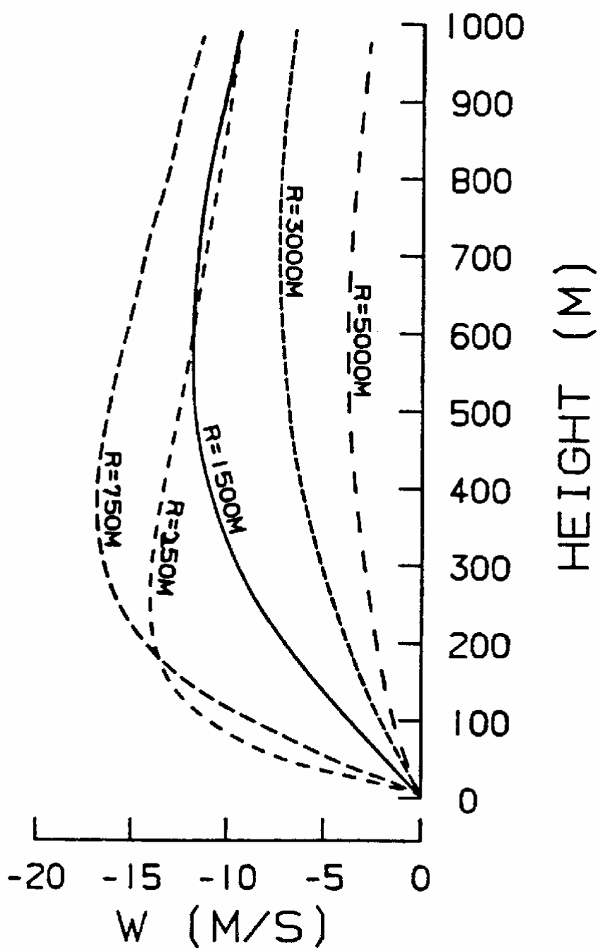
Figure 3 Vertical Profile of Microburst Downflow
