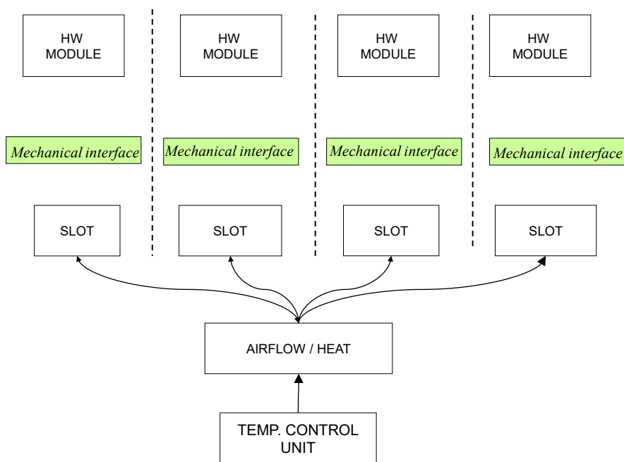
Figure 14: CLASS RH Cooling elements relationship
