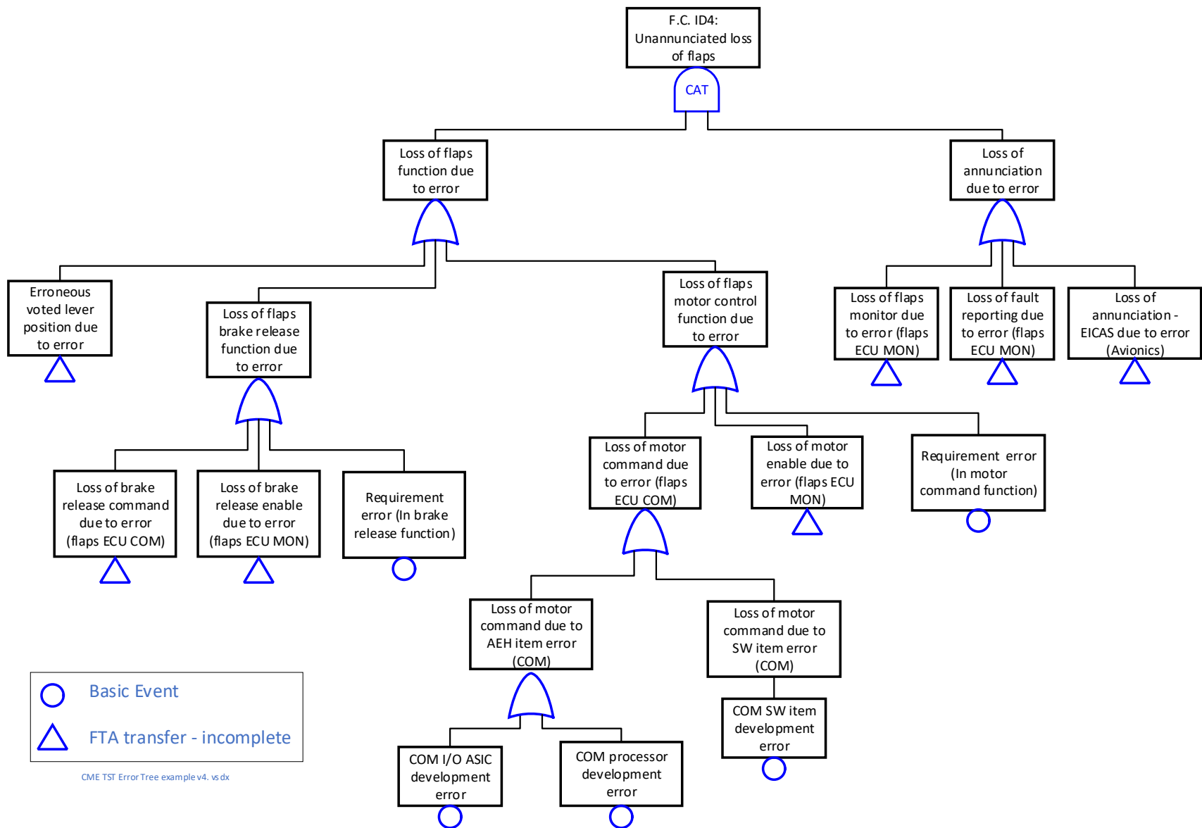
Figure 7 - Error fault tree partial example
