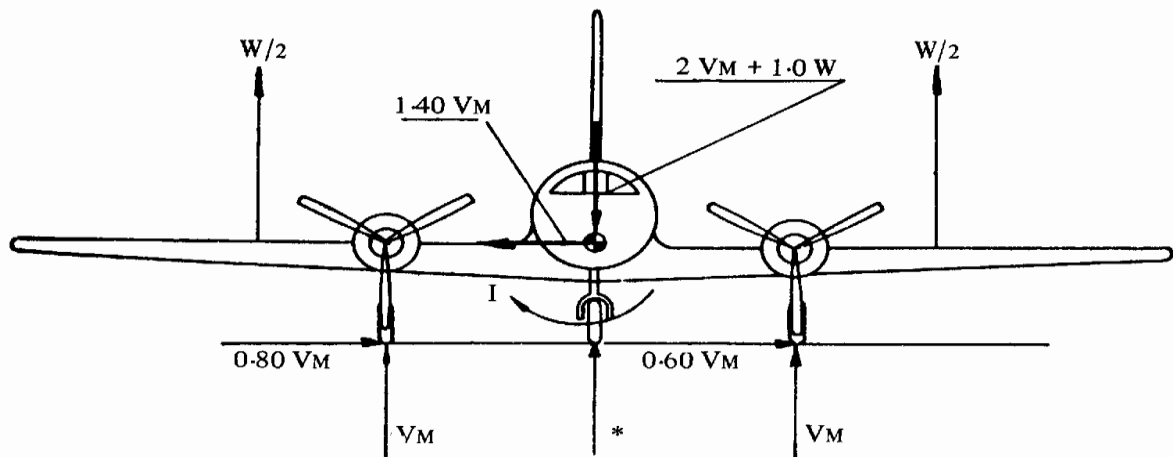
FIGURE 4 ONE-WHEEL LANDING
