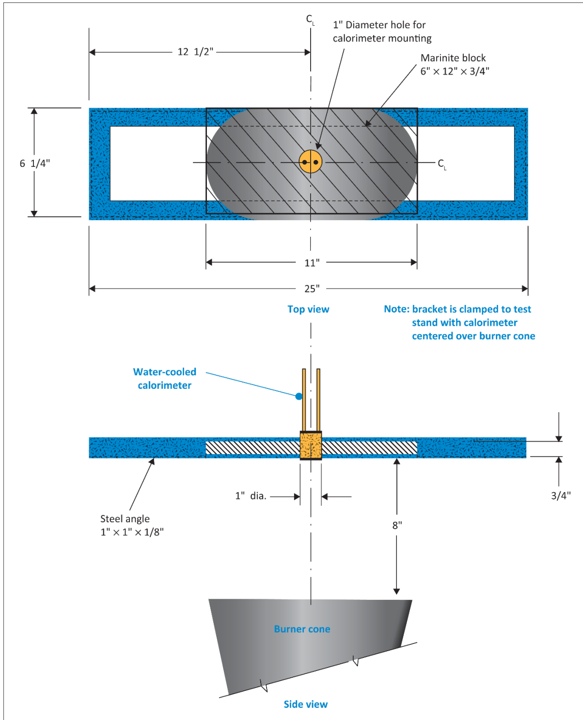
FIGURE 2 CALORIMETER BRACKET
