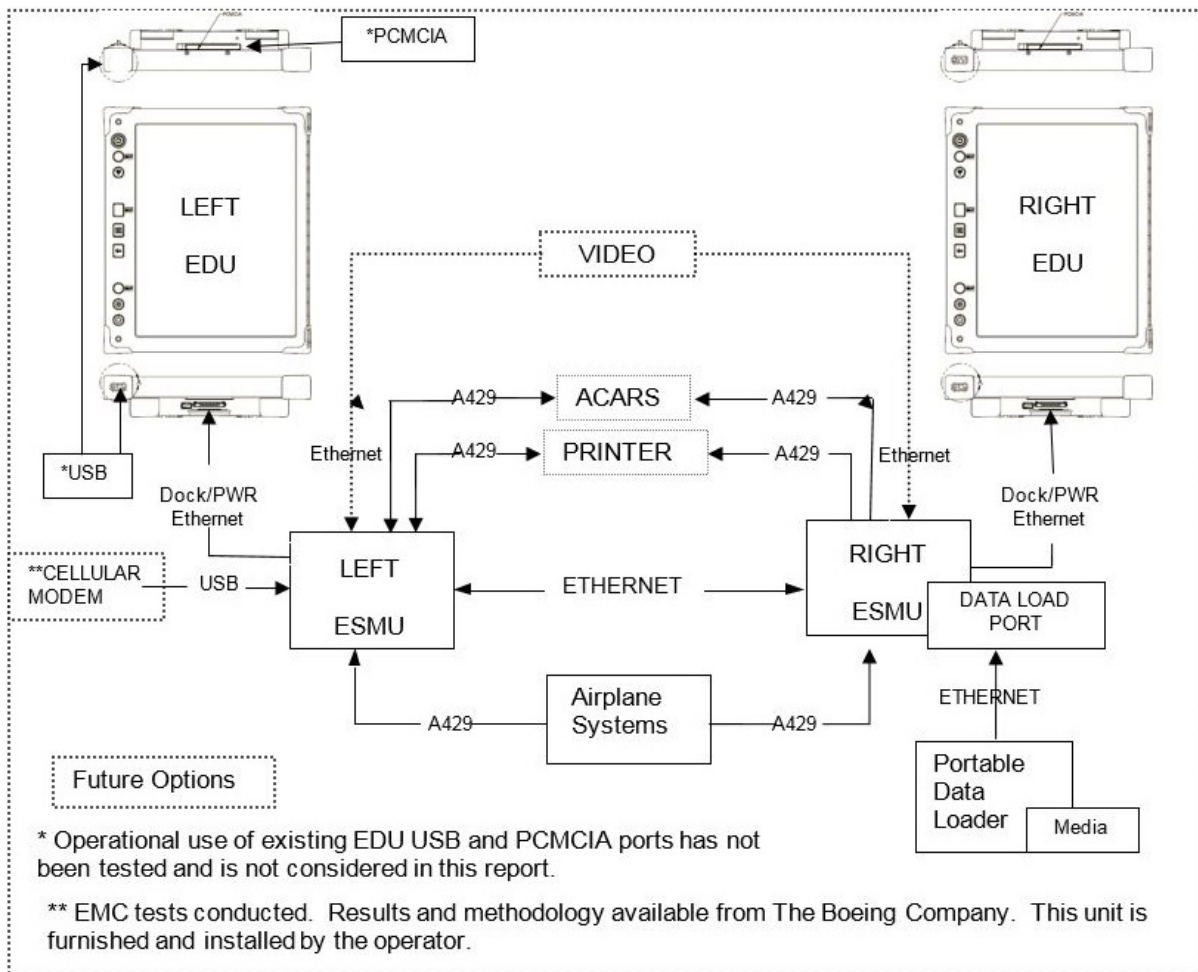
Figure 2-6. EFB Basic Plus Optional Equipment Installation Schematic (737 NG)
