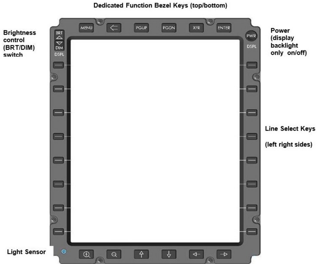
Figure 2-2. EFB Display Unit
